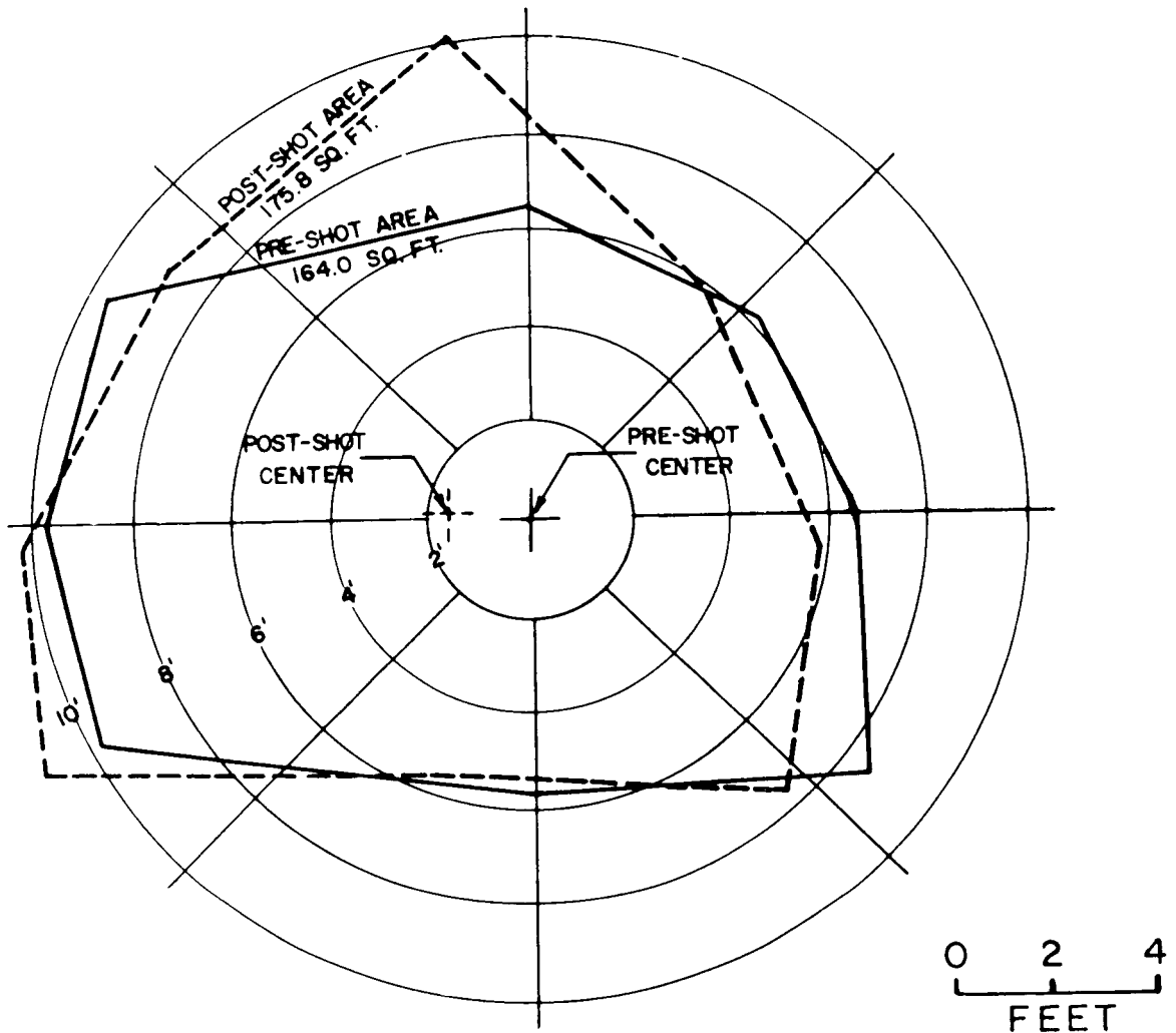
Fig. 11 — Preshot and postshot cross sections, drift U12e, station 11+20.
